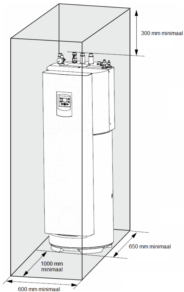
Techneco Loria Duo
